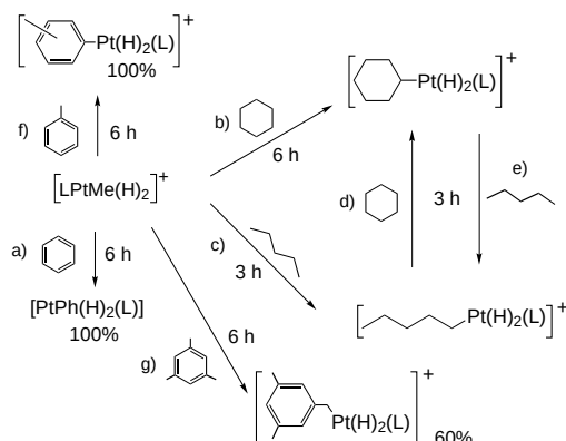
Scheme 2. Reactions of [\text{LPtMe}(\text{H})_2]^+ . See text for details.
